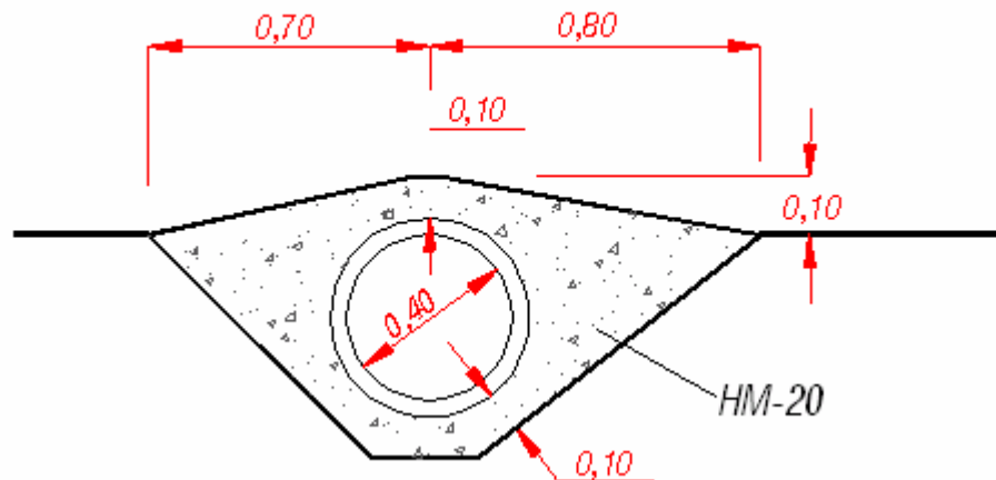
Paso salvacunetas
